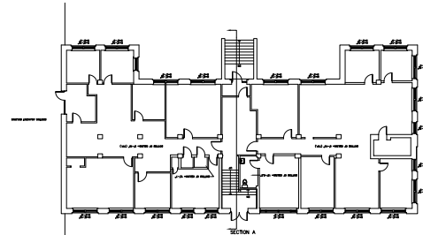
2 FIRST FLOOR PLAN — BLDG 75 SCALE: 1/16" = 1' - 0"
