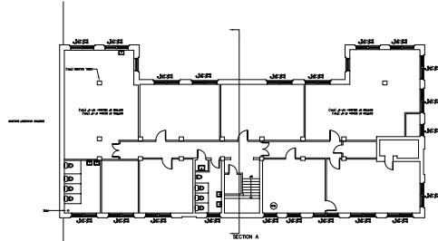
1 BASEMENT PLAN — BLDG 75 SCALE: 1/16" = 1' - 0"
